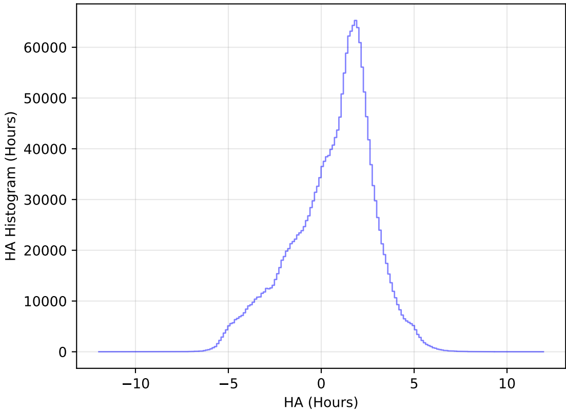
too_elab_r16_d3_giz_v3.4_10yrs WFD all bands: HA Histogram
