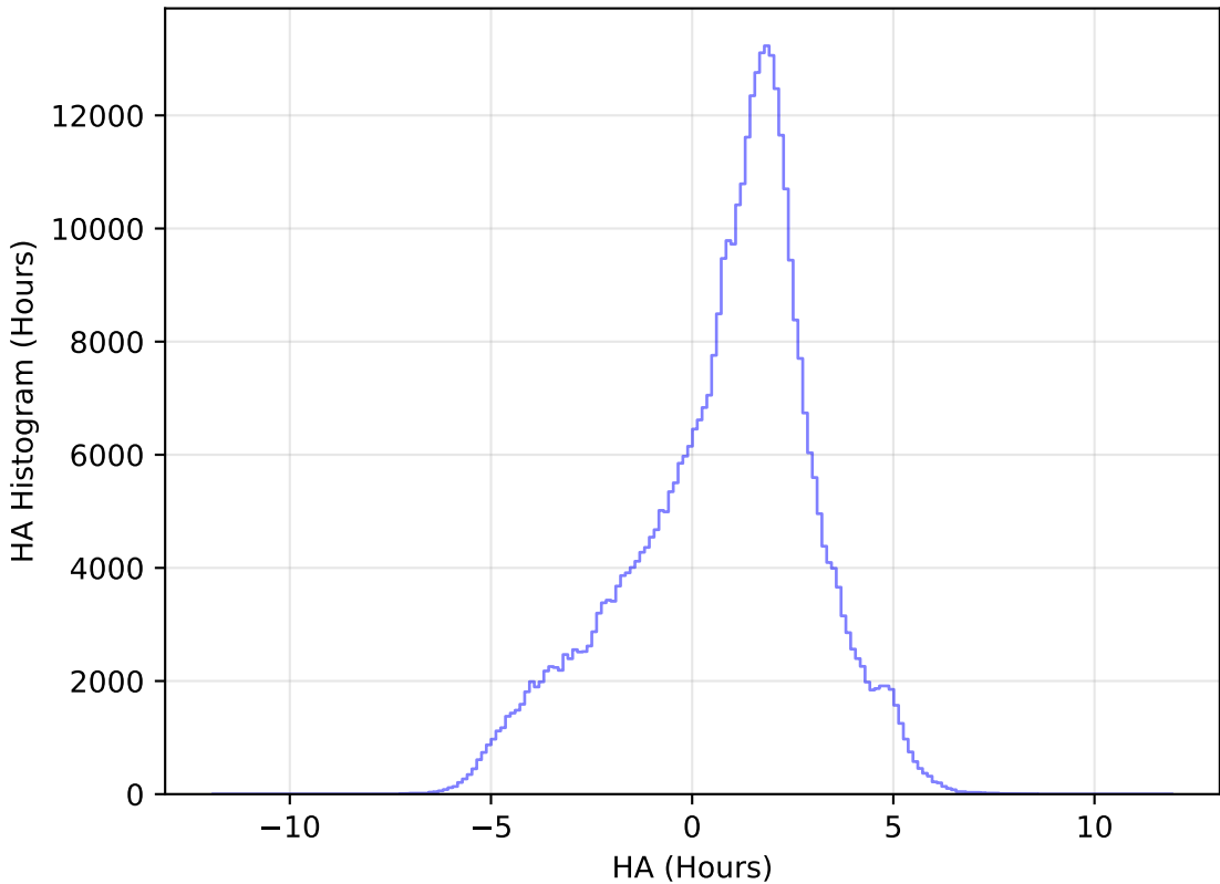
too_elab_r16_d3_giz_v3.4_10yrs All sky z band: HA Histogram
