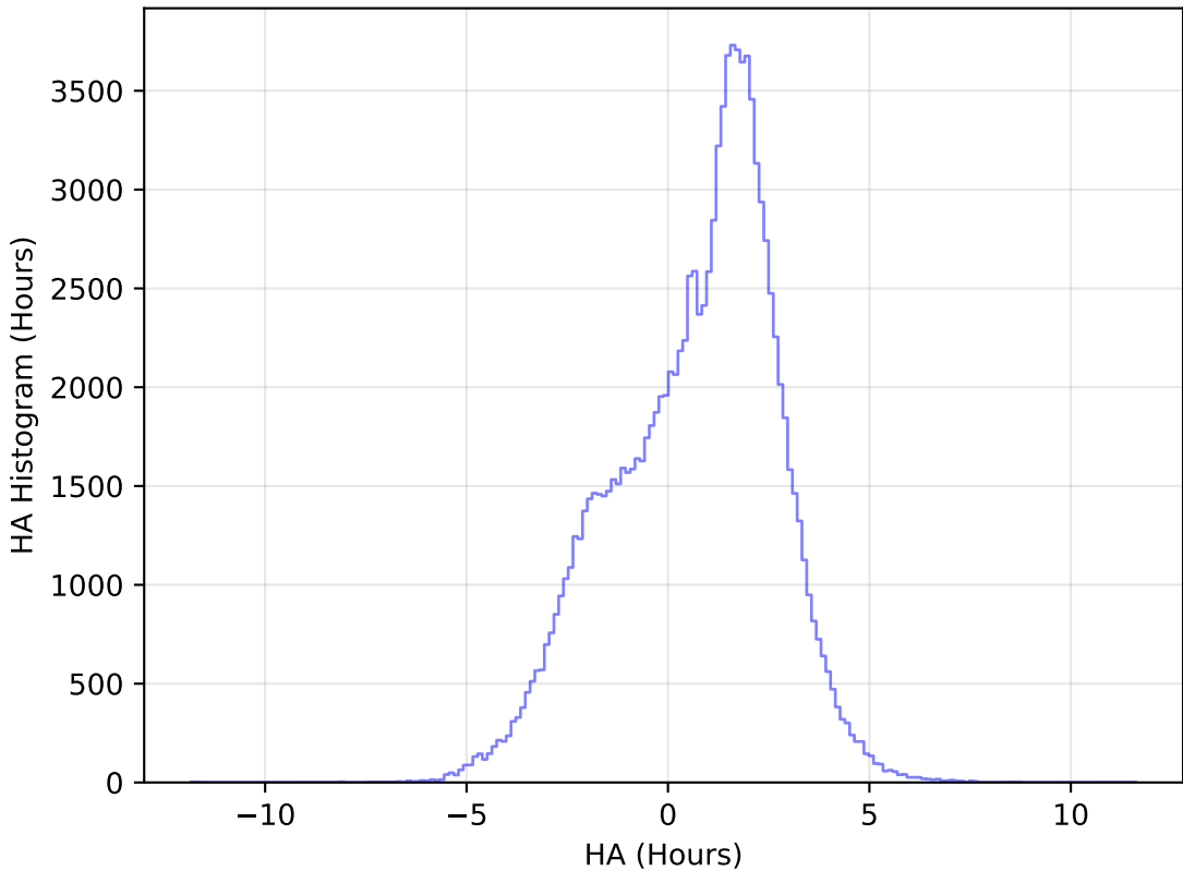
too_elab_r16_d3_giz_v3.4_10yrs All sky u band: HA Histogram
