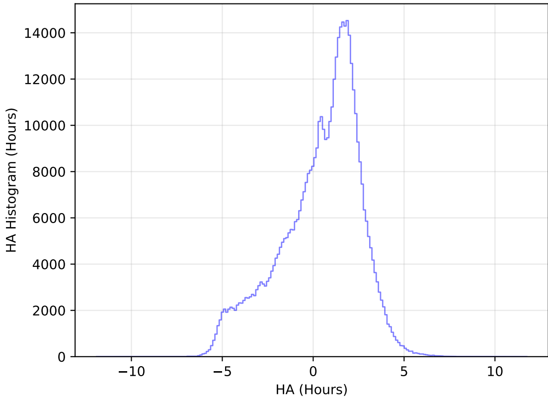
too_elab_r16_d3_giz_v3.4_10yrs All sky r band: HA Histogram
