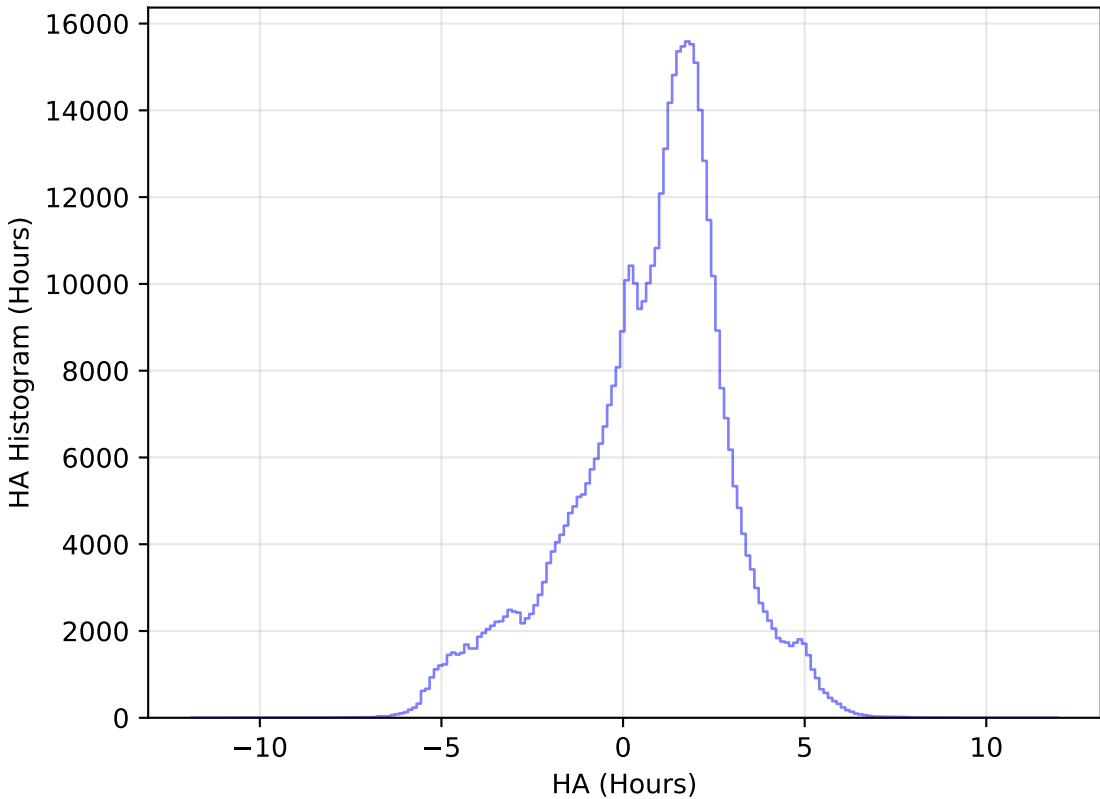
too_elab_r16_d3_giz_v3.4_10yrs All sky i band: HA Histogram
