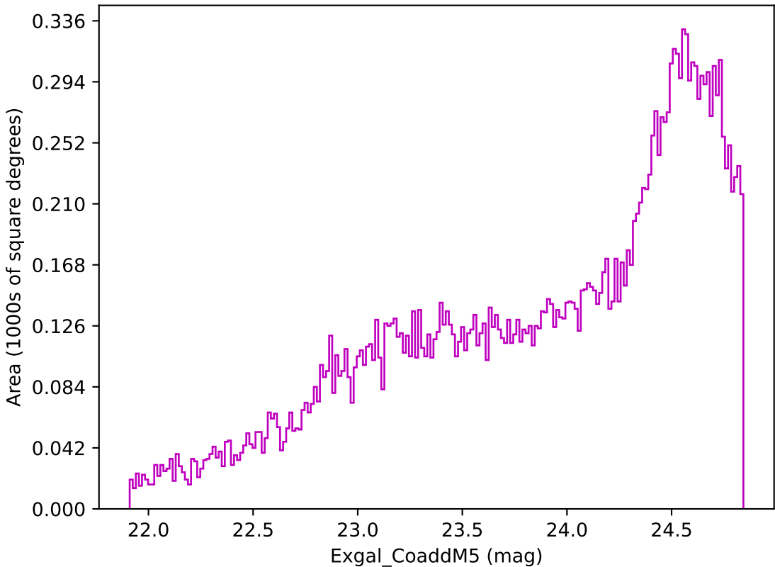
too_elab_r16_d3_giz_v3.4_10yrs Yr 3-4 z band: Exgal_CoaddM5
