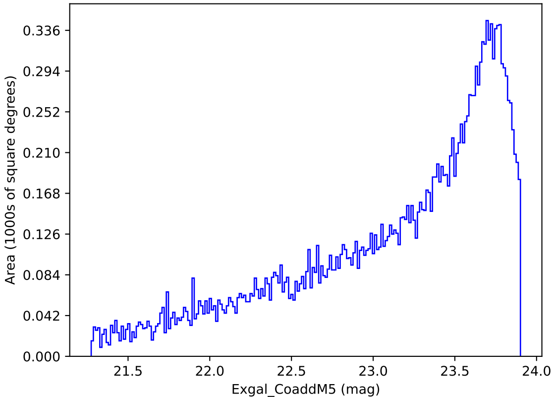
too_elab_r16_d3_giz_v3.4_10yrs Yr 3-4 y band: Exgal_CoaddM5
