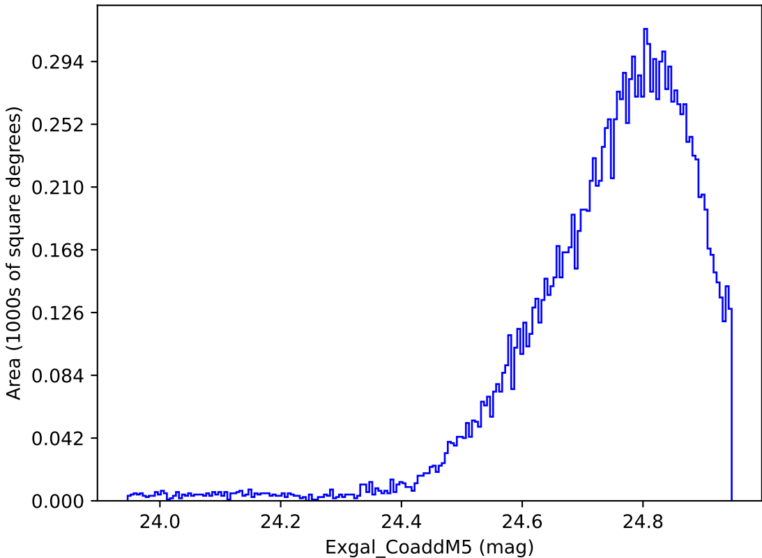
too_elab_r16_d3_giz_v3.4_10yrs WFD y band: Exgal_CoaddM5
