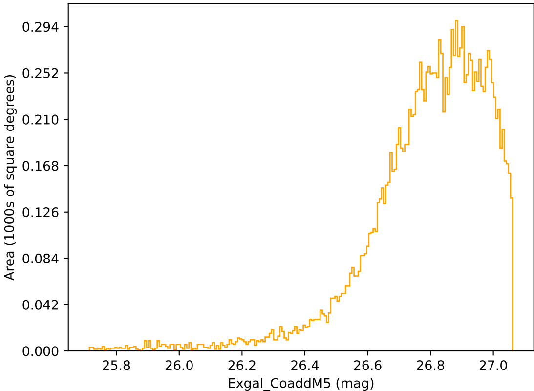
too_elab_r16_d3_giz_v3.4_10yrs WFD r band: Exgal_CoaddM5
