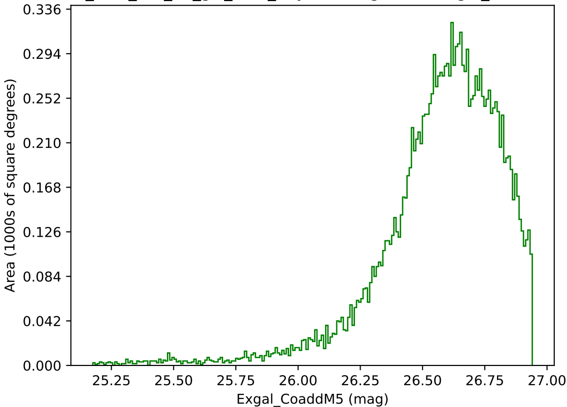
too_elab_r16_d3_giz_v3.4_10yrs WFD g band: Exgal_CoaddM5
