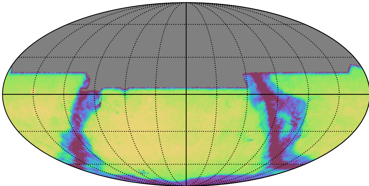
too_elab_r16_d3_giz_v3.4_10yrs All sky y band: Exgal_CoaddM5
