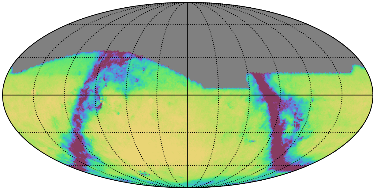
too_elab_r16_d3_giz_v3.4_10yrs All sky g band: Exgal_CoaddM5
