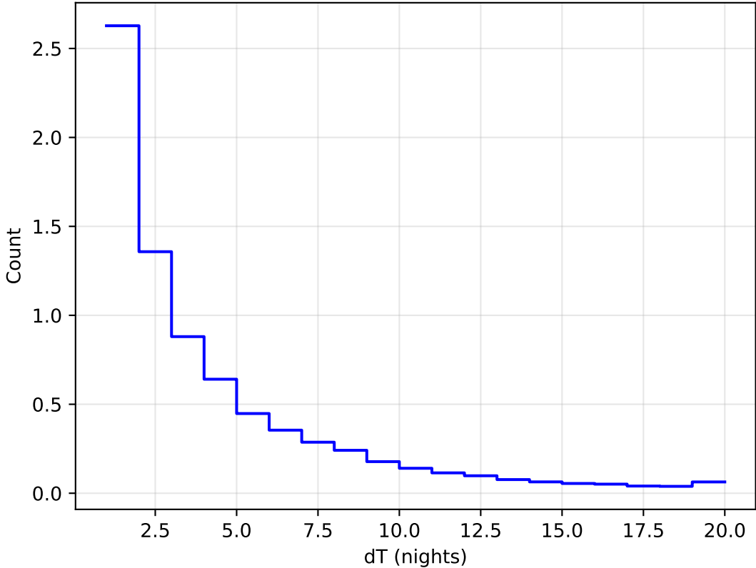
too_elab_r16_d3_giz_v3.4_10yrs WFD all bands: DeltaNight Histogram
