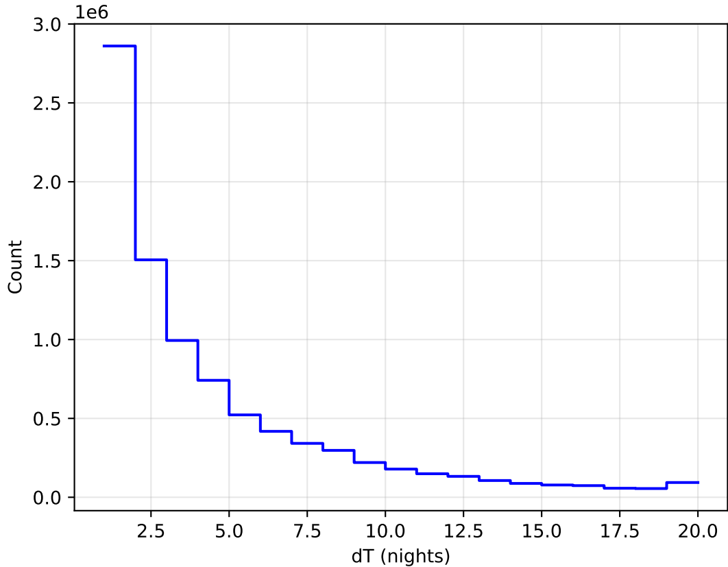
too_elab_r16_d3_giz_v3.4_10yrs All sky all bands: DeltaNight Histogram
