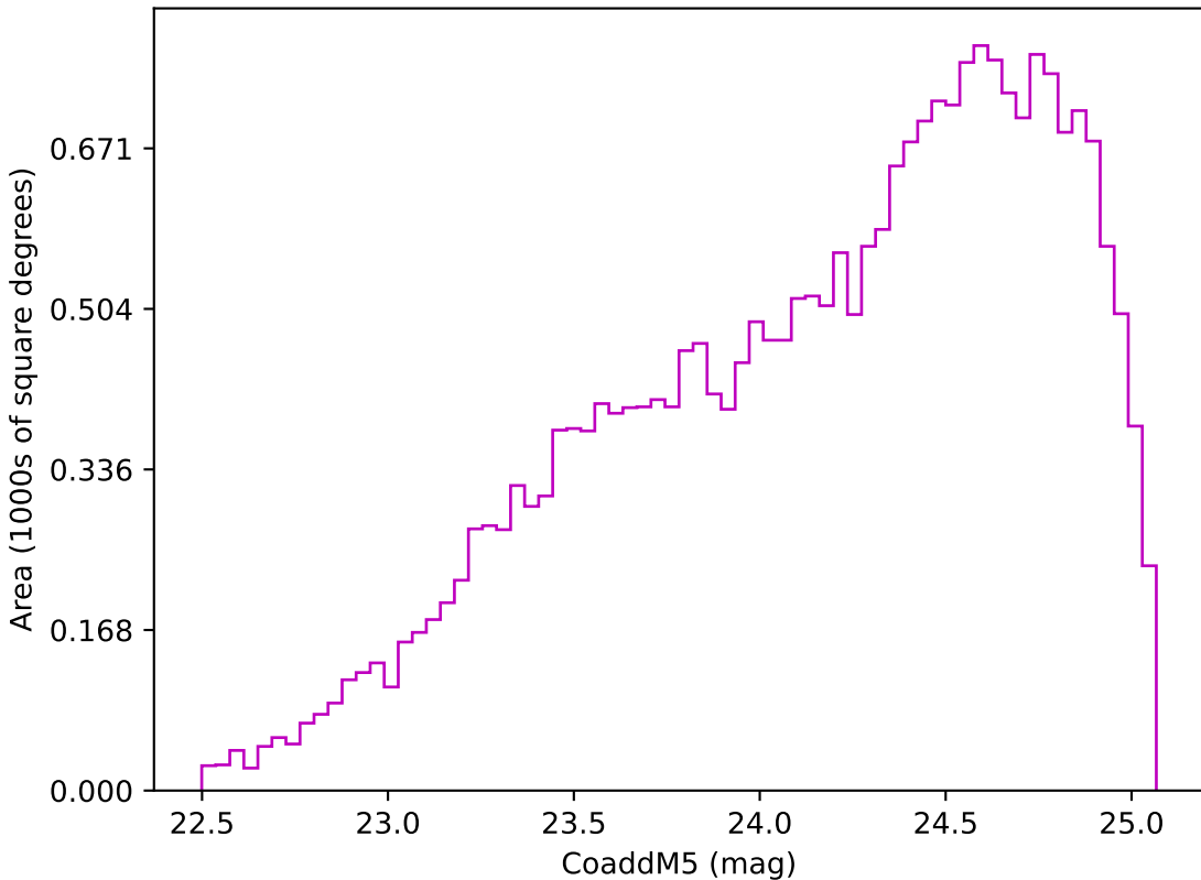
too_elab_r16_d3_giz_v3.4_10yrs Yr 3-4 z band: CoaddM5
