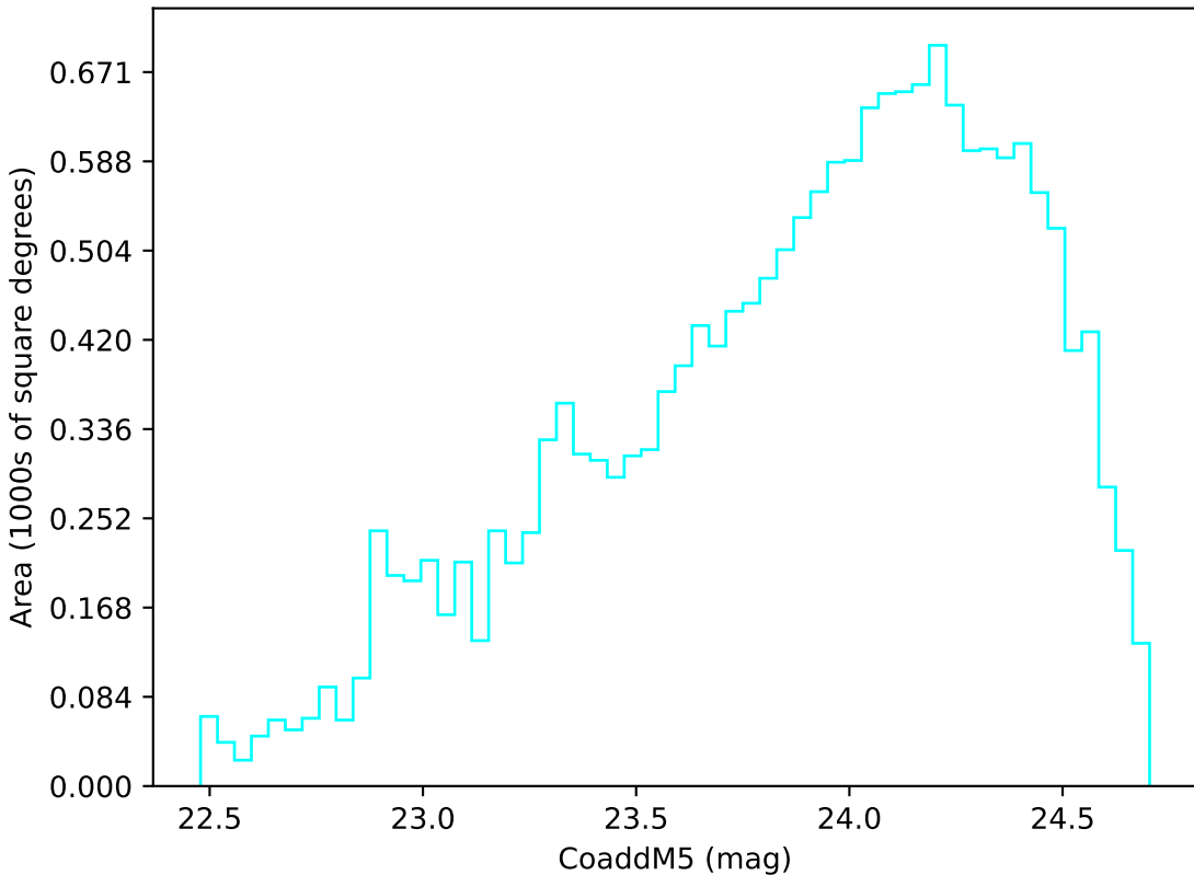
too_elab_r16_d3_giz_v3.4_10yrs Yr 3-4 u band: CoaddM5
