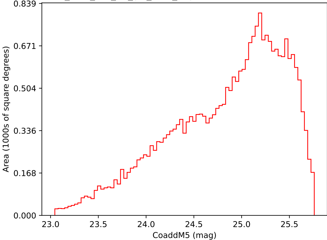
too_elab_r16_d3_giz_v3.4_10yrs Yr 3-4 i band: CoaddM5
