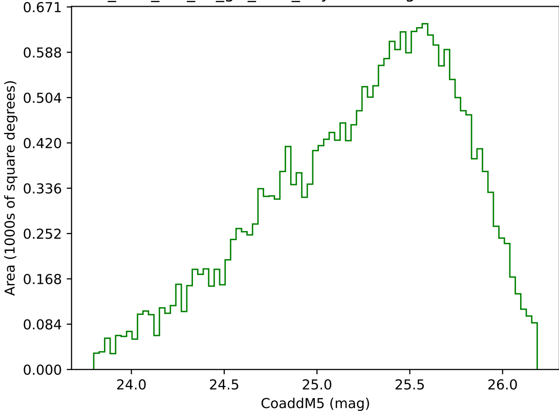
too_elab_r16_d3_giz_v3.4_10yrs Yr 3-4 g band: CoaddM5
