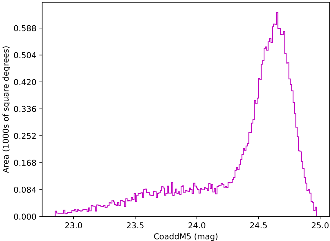
too_elab_r16_d3_giz_v3.4_10yrs Yr 1 z band: CoaddM5
