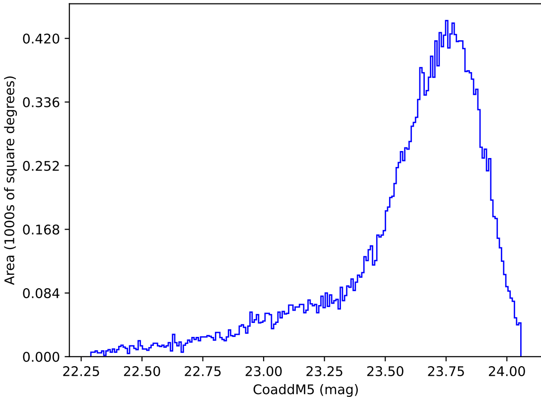
too_elab_r16_d3_giz_v3.4_10yrs Yr 1 y band: CoaddM5
