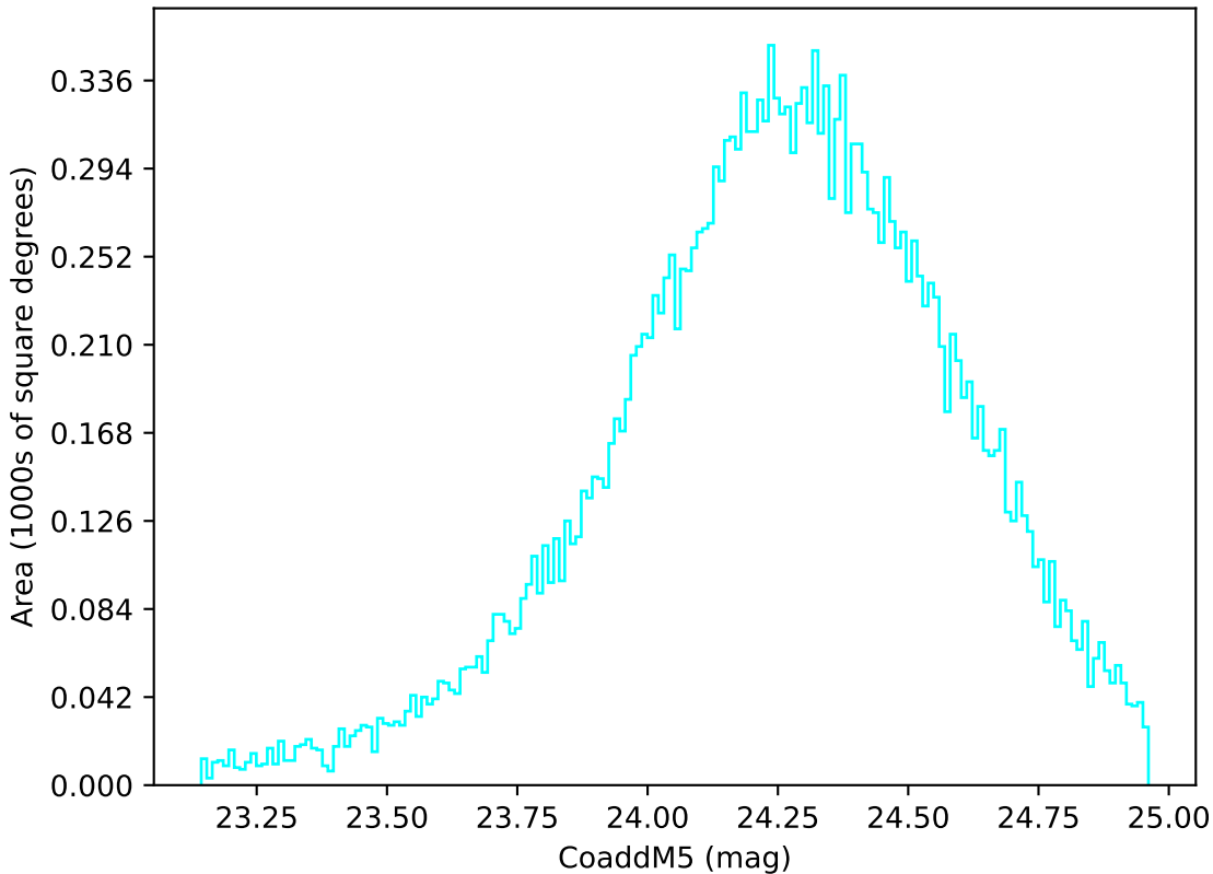
too_elab_r16_d3_giz_v3.4_10yrs Yr 1 u band: CoaddM5
