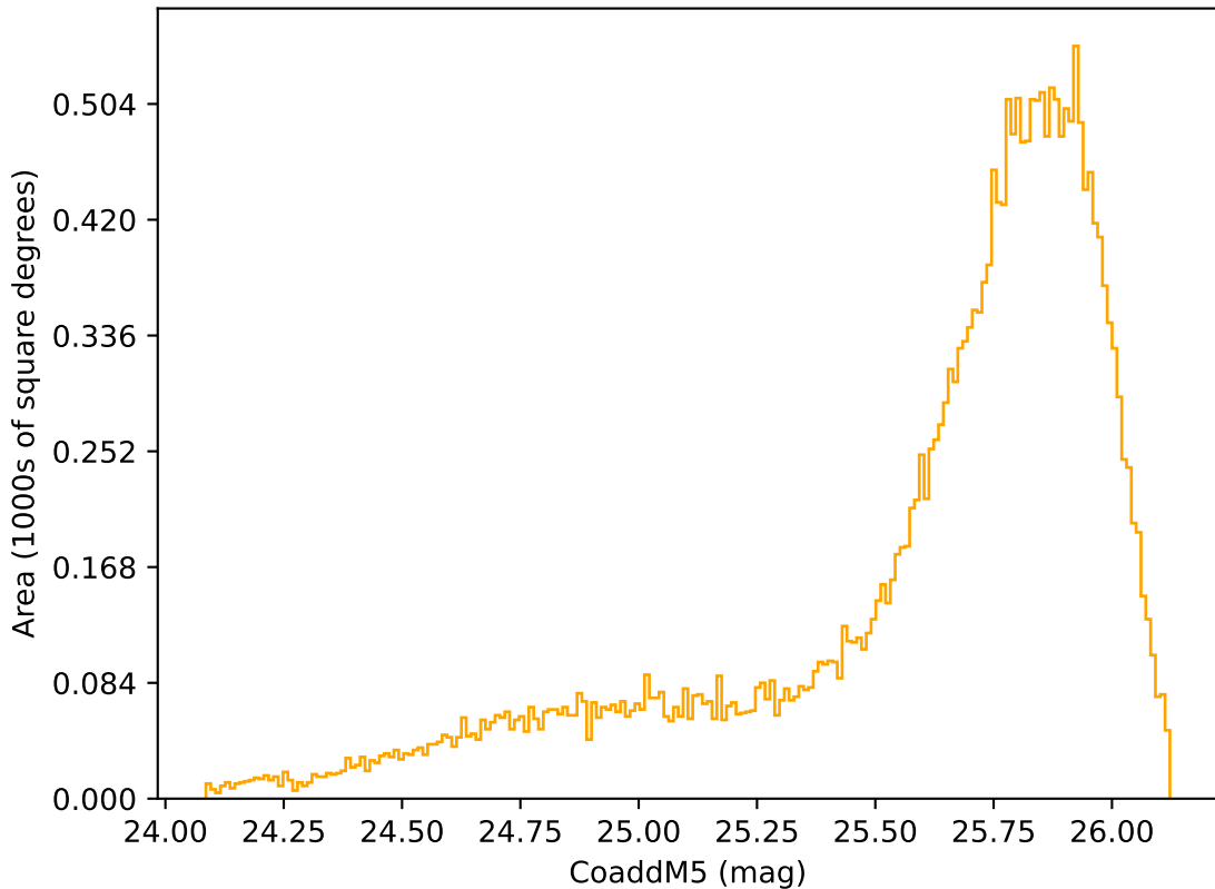
too_elab_r16_d3_giz_v3.4_10yrs Yr 1 r band: CoaddM5
