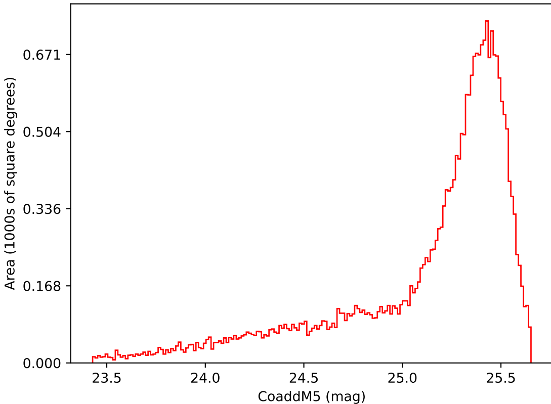
too_elab_r16_d3_giz_v3.4_10yrs Yr 1 i band: CoaddM5
