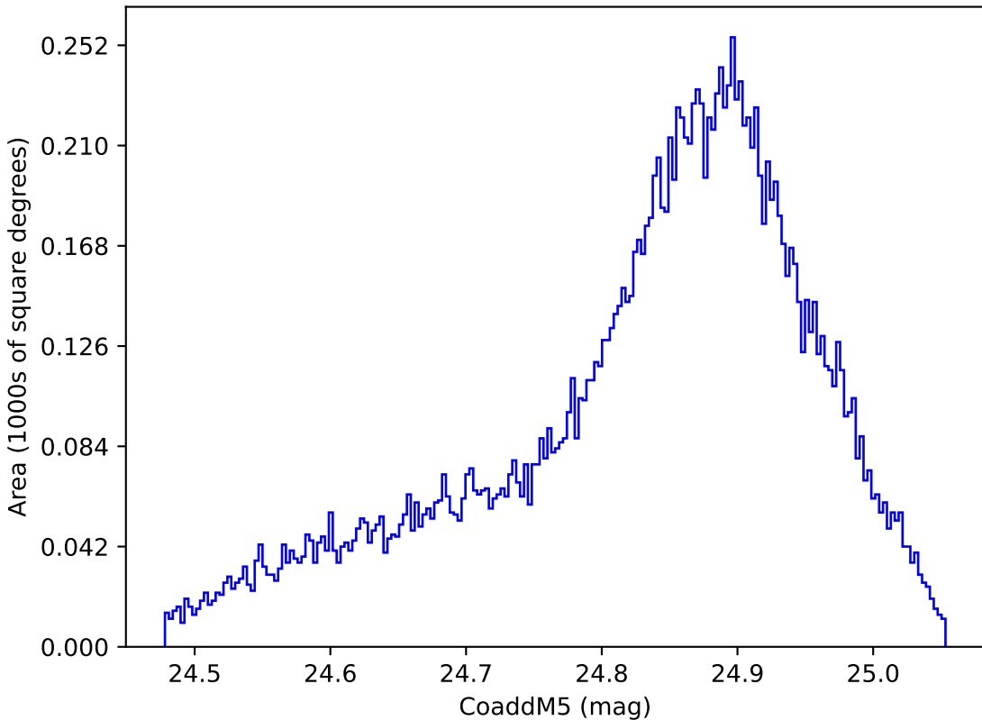
too_elab_r16_d3_giz_v3.4_10yrs WFD y band: CoaddM5
