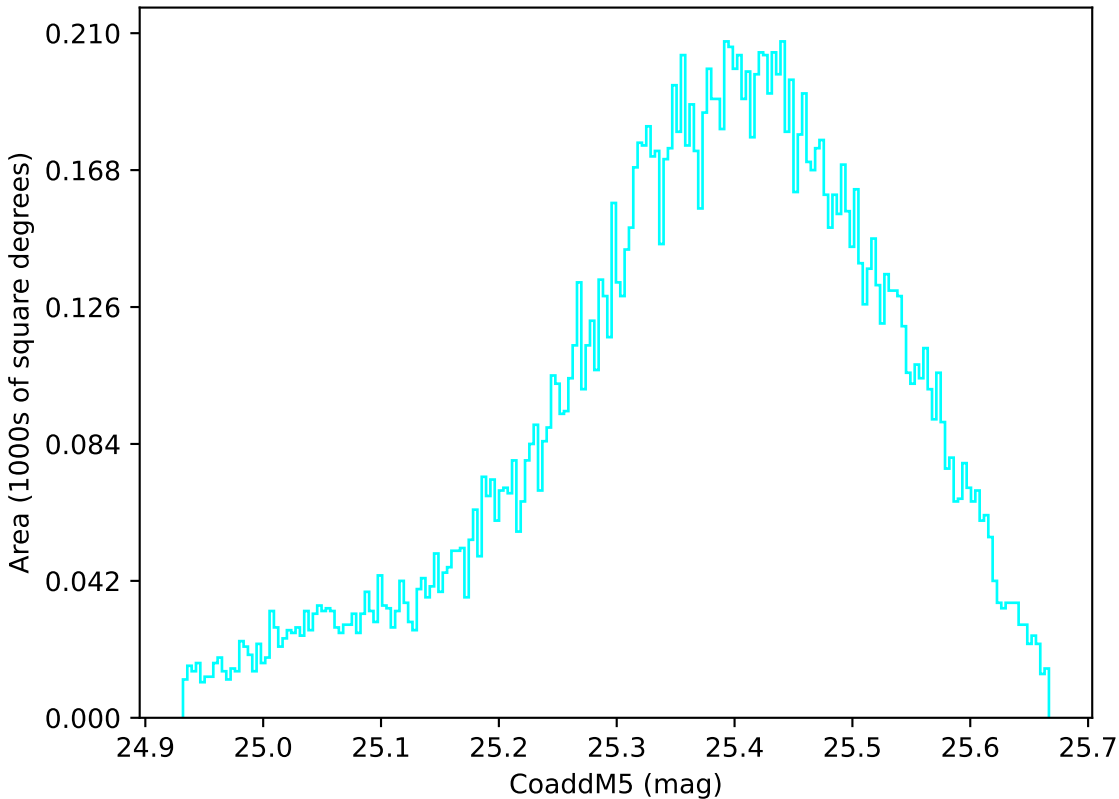
too_elab_r16_d3_giz_v3.4_10yrs WFD u band: CoaddM5
