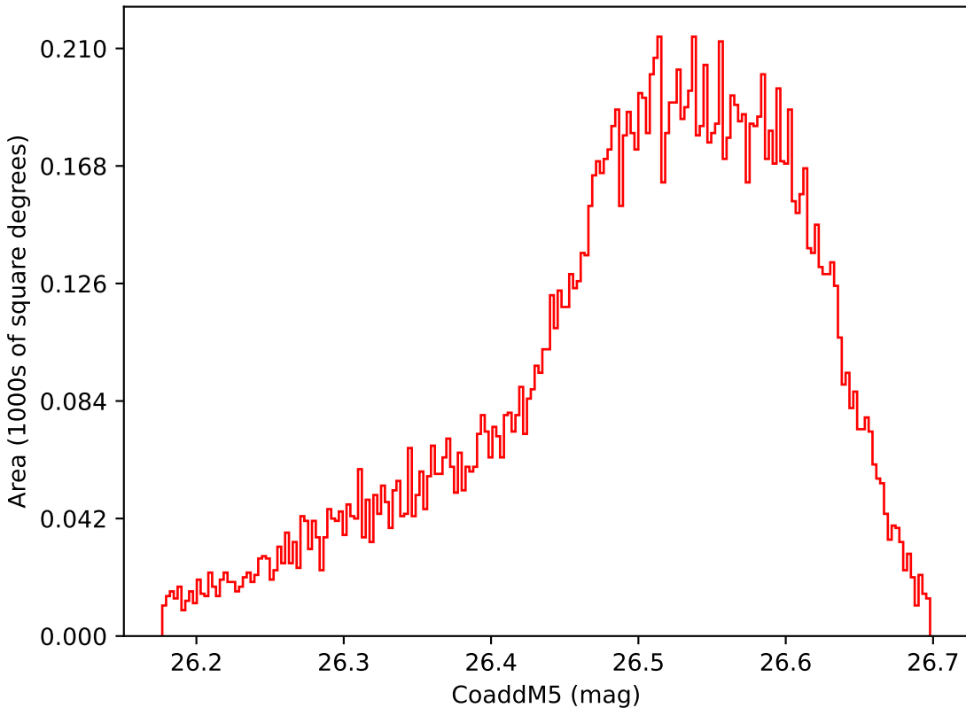
too_elab_r16_d3_giz_v3.4_10yrs WFD i band: CoaddM5
