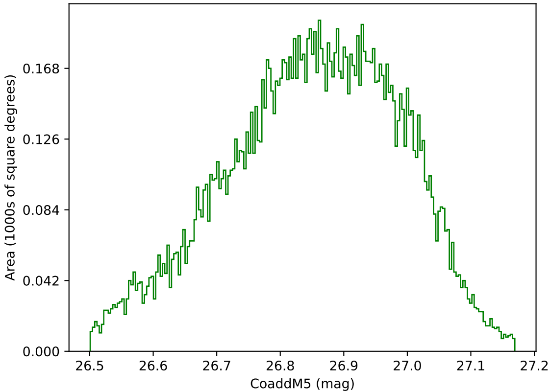
too_elab_r16_d3_giz_v3.4_10yrs WFD g band: CoaddM5
