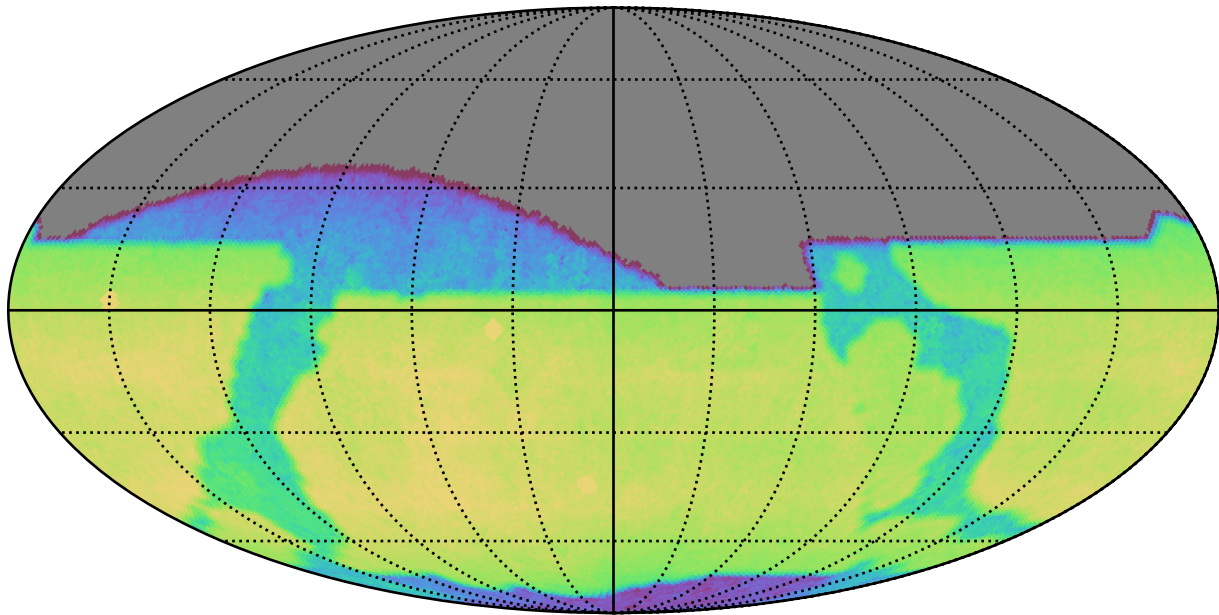
too_elab_r16_d3_giz_v3.4_10yrs All sky z band: CoaddM5
