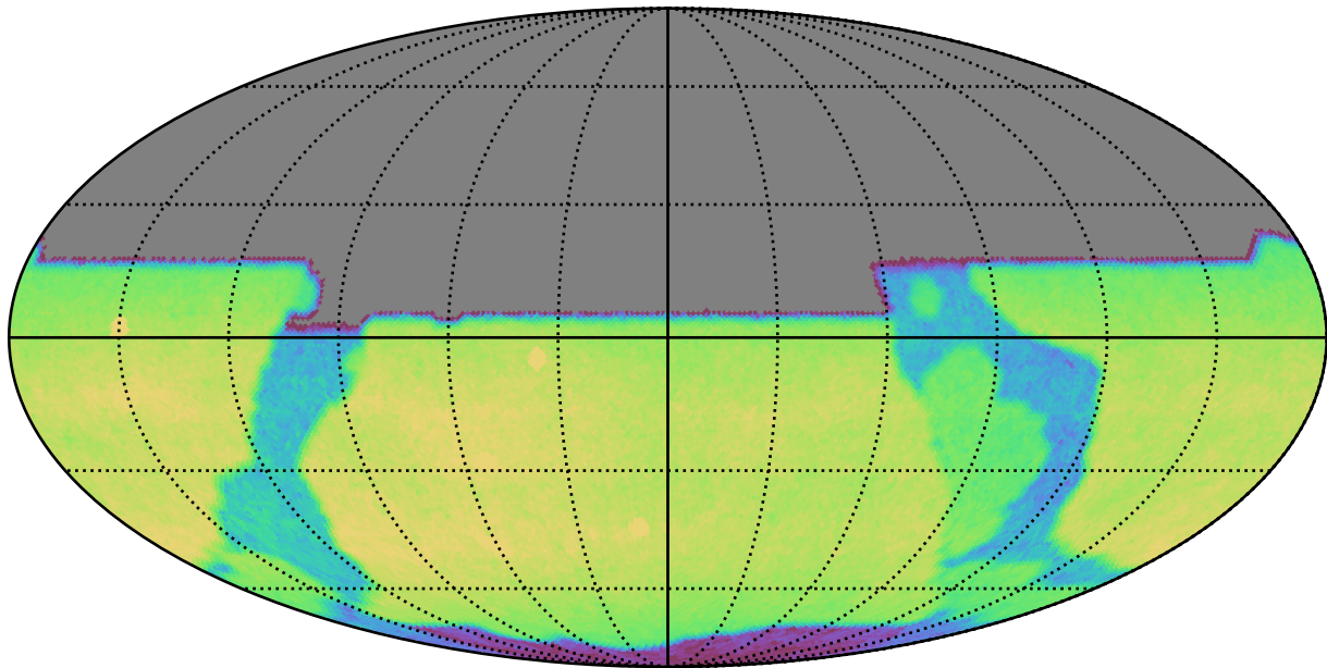
too_elab_r16_d3_giz_v3.4_10yrs All sky y band: CoaddM5
