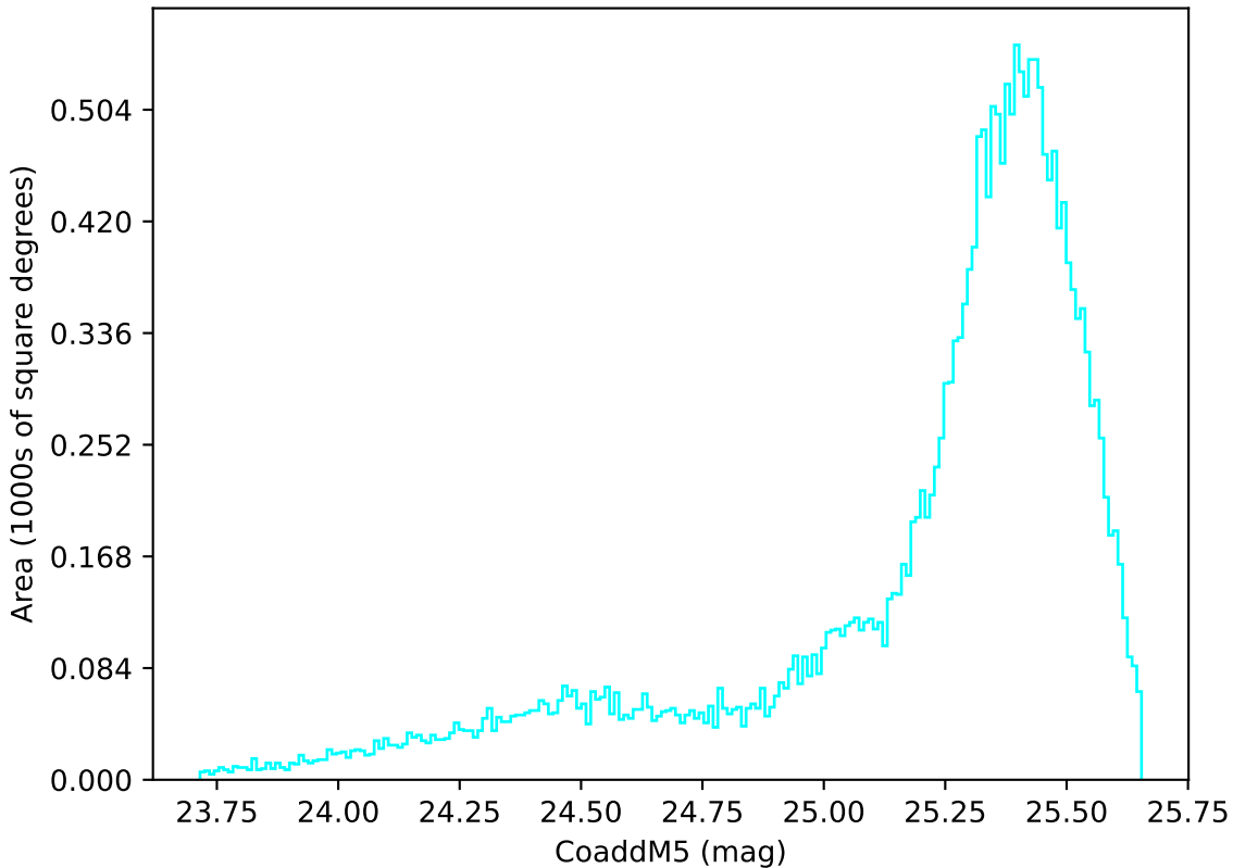
too_elab_r16_d3_giz_v3.4_10yrs All sky u band: CoaddM5
