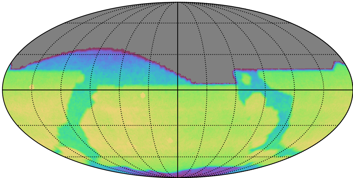
too_elab_r16_d3_giz_v3.4_10yrs All sky r band: CoaddM5
