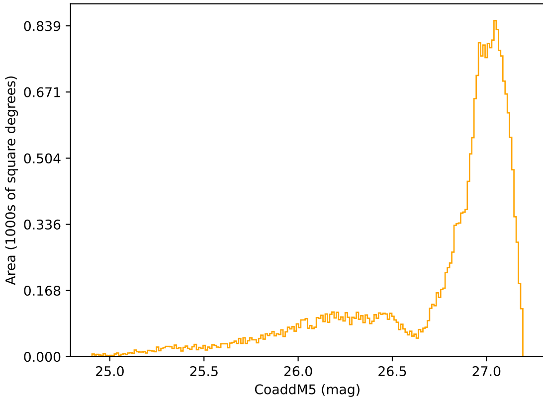
too_elab_r16_d3_giz_v3.4_10yrs All sky r band: CoaddM5
