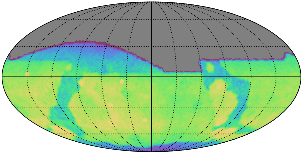
too_elab_r16_d3_giz_v3.4_10yrs All sky g band: CoaddM5
