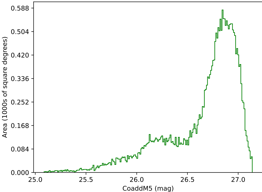
too_elab_r16_d3_giz_v3.4_10yrs All sky g band: CoaddM5
