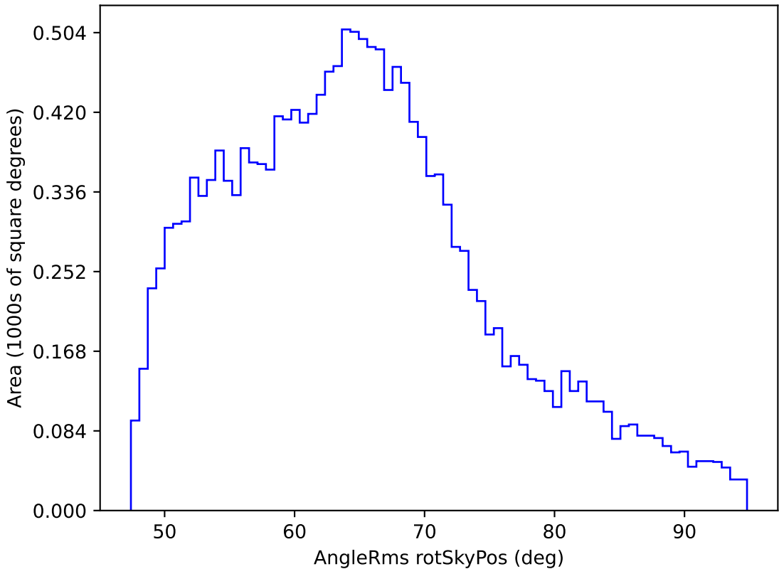
too_elab_r16_d3_giz_v3.4_10yrs WFD z band: AngleRms rotSkyPos
