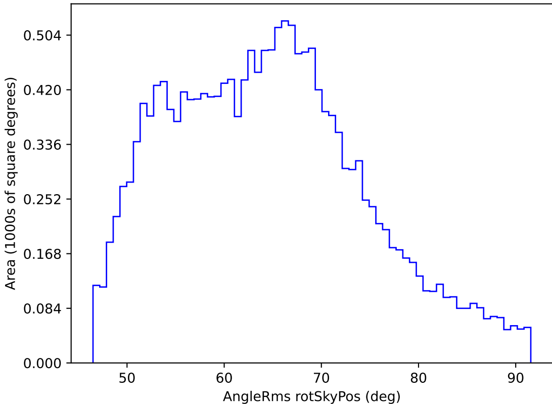
too_elab_r16_d3_giz_v3.4_10yrs WFD i band: AngleRms rotSkyPos
