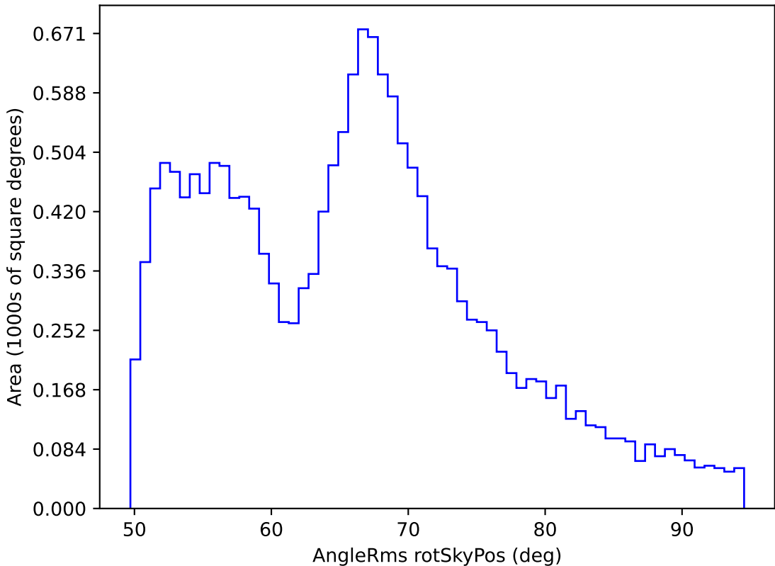
too_elab_r16_d3_giz_v3.4_10yrs WFD all bands: AngleRms rotSkyPos
