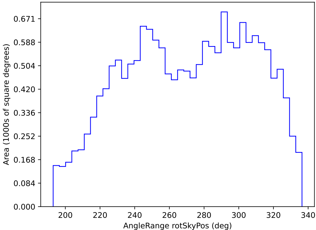
too_elab_r16_d3_giz_v3.4_10yrs WFD y band: AngleRange rotSkyPos
