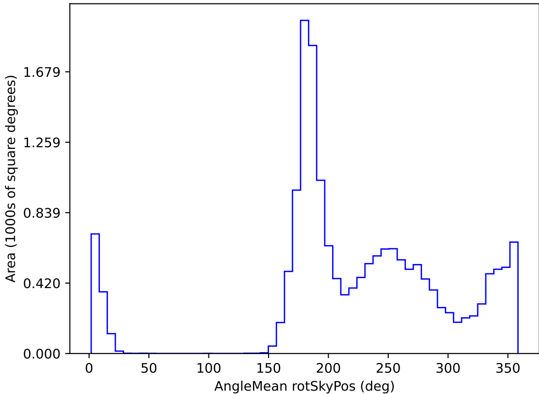
too_elab_r16_d3_giz_v3.4_10yrs WFD y band: AngleMean rotSkyPos
