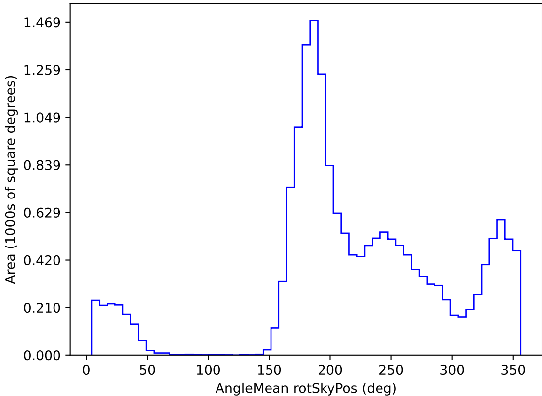
too_elab_r16_d3_giz_v3.4_10yrs WFD u band: AngleMean rotSkyPos
