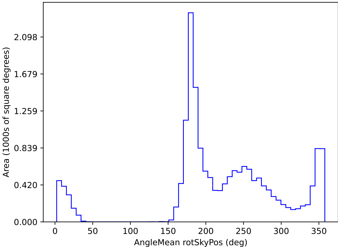
too_elab_r16_d3_giz_v3.4_10yrs WFD i band: AngleMean rotSkyPos
