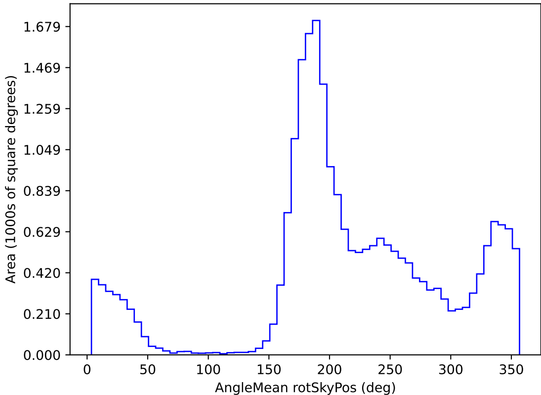
too_elab_r16_d3_giz_v3.4_10yrs All sky u band: AngleMean rotSkyPos
