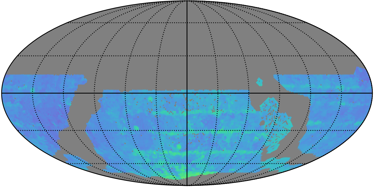
too_elab_r16_d3_giz_v3.4_10yrs WFD z band: 80thPercentile Season Length
