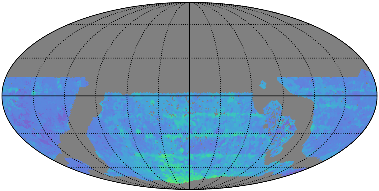
too_elab_r16_d3_giz_v3.4_10yrs WFD y band: 80thPercentile Season Length
