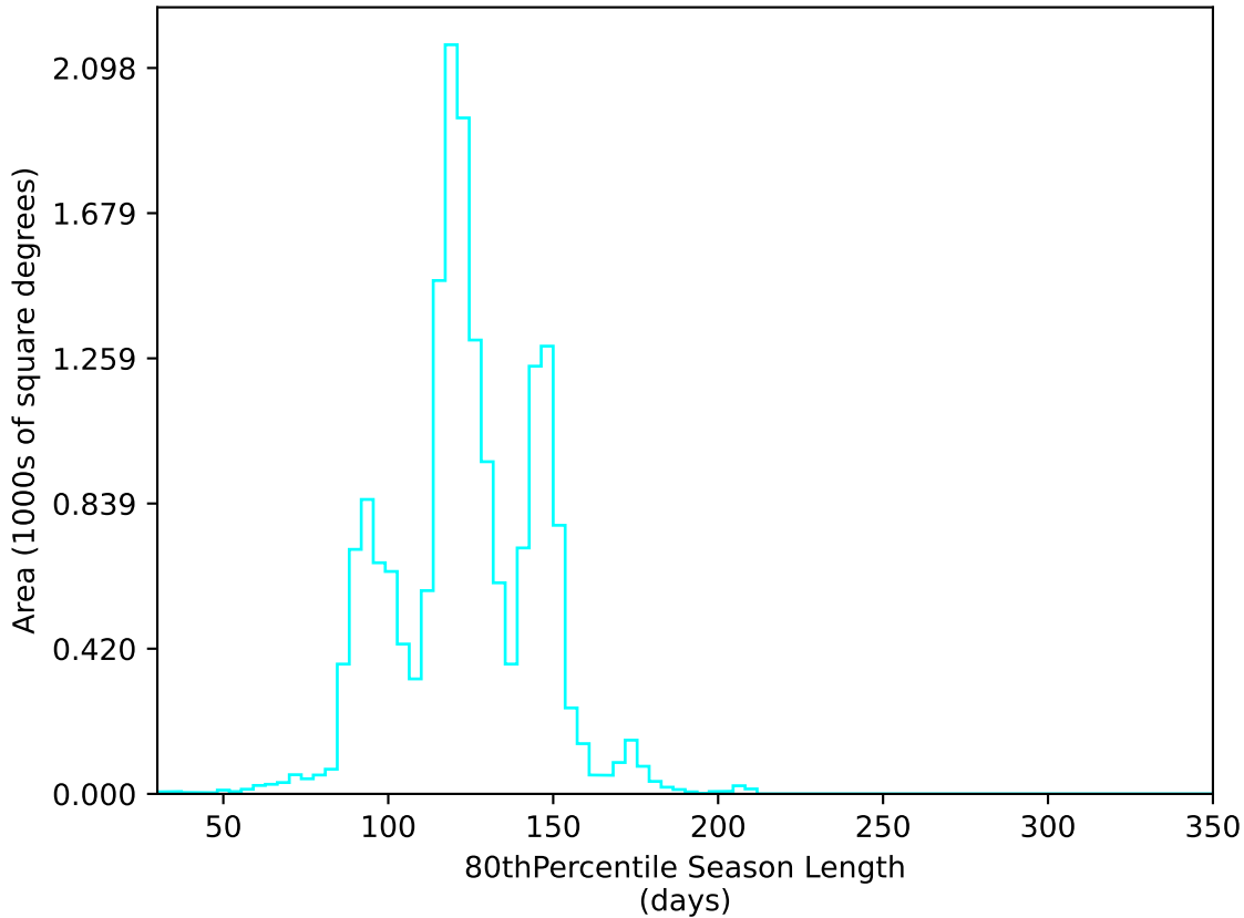
too_elab_r16_d3_giz_v3.4_10yrs WFD u band: 80thPercentile Season Length
