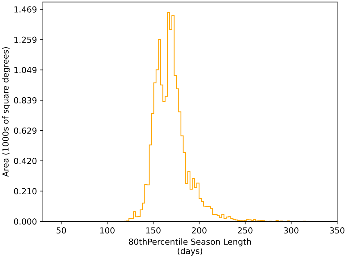
too_elab_r16_d3_giz_v3.4_10yrs WFD r band: 80thPercentile Season Length
