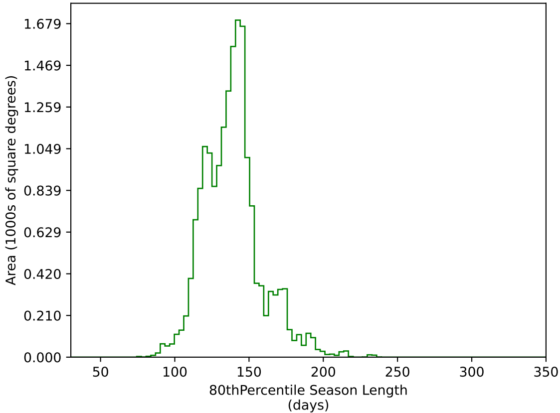
too_elab_r16_d3_giz_v3.4_10yrs WFD g band: 80thPercentile Season Length
