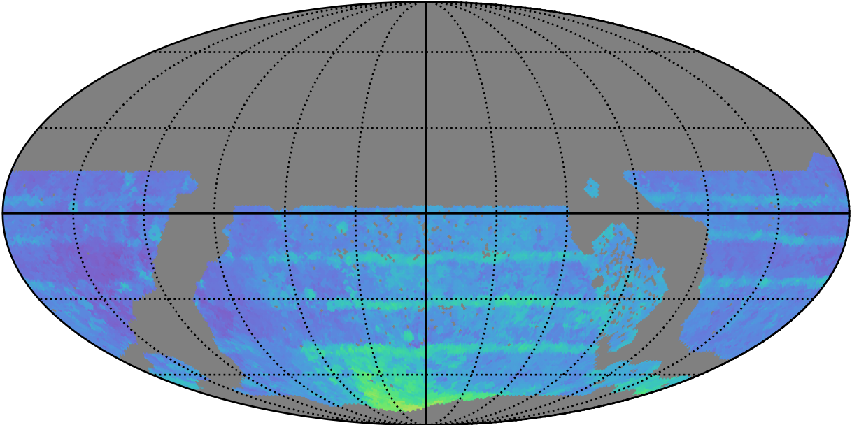
too_elab_r16_d3_giz_v3.4_10yrs WFD all bands: 80thPercentile Season Length
