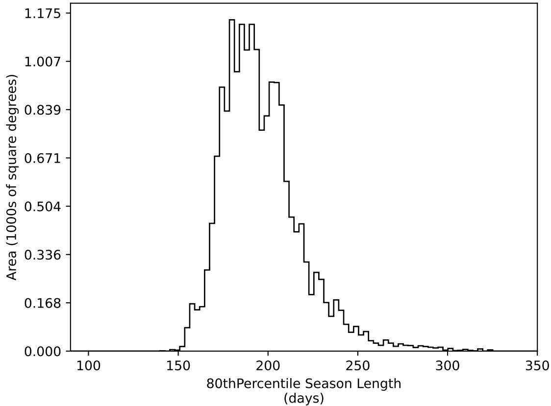
too_elab_r16_d3_giz_v3.4_10yrs WFD all bands: 80thPercentile Season Length
