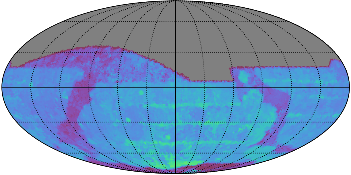
too_elab_r16_d3_giz_v3.4_10yrs All sky z band: 80thPercentile Season Length
